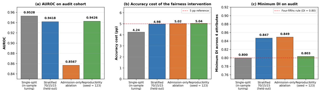
Comparison of validation protocols on Texas-100X audit cohort
