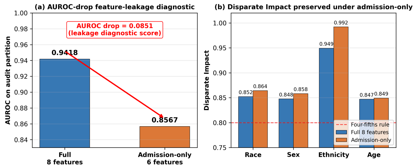
Feature-leakage diagnostic on the audit partition
